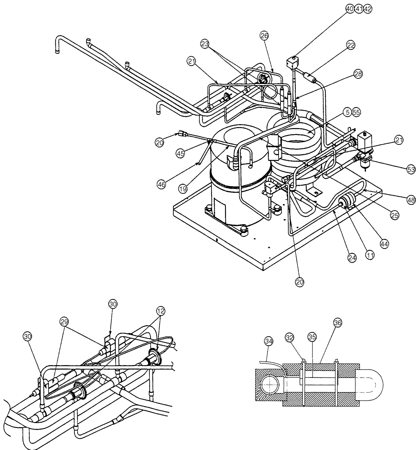
DETAILED THERMISTOR ATTACHMENT
